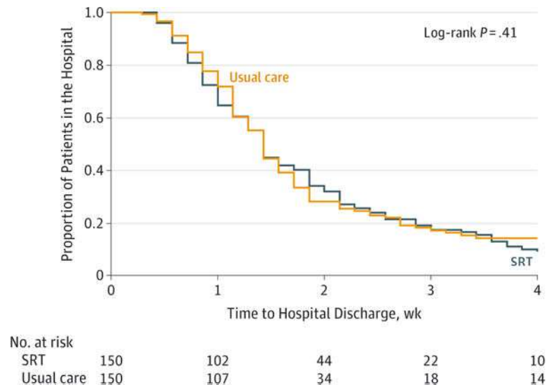
Figure 2. Length of Stay for Patients With Acute Respiratory Failure Receiving SRT vs Usual Care
